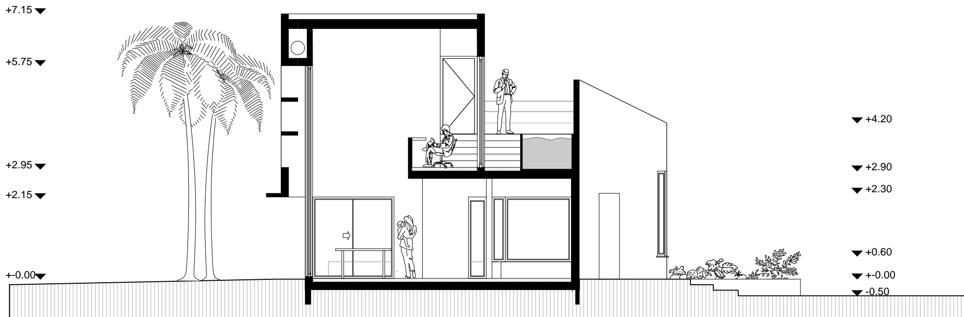
B-B section
