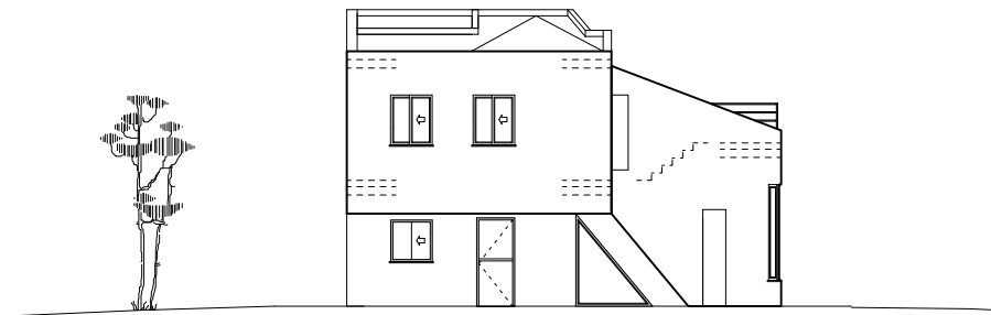
east facade
