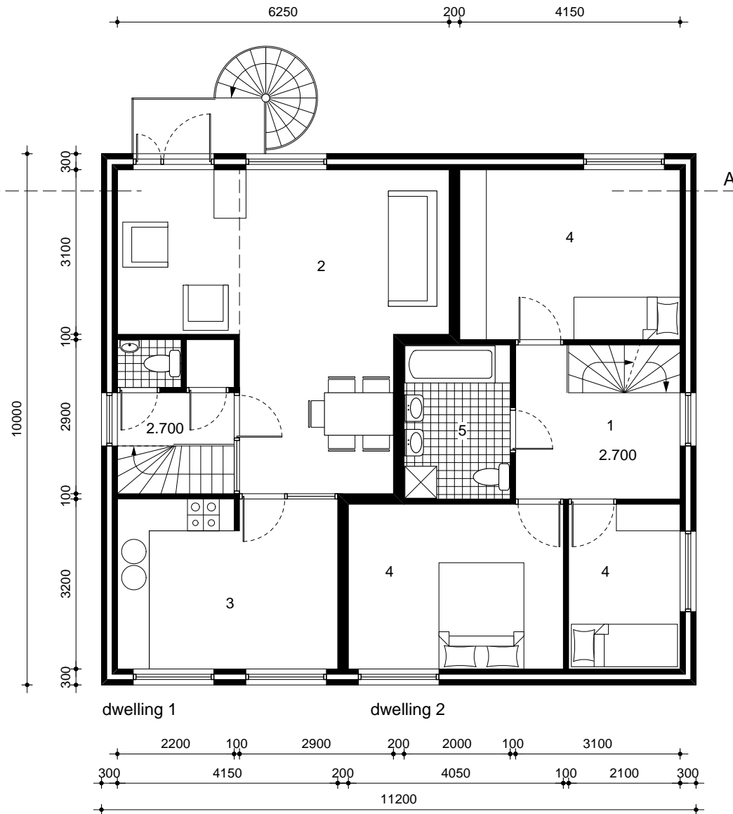
First floor 1:100
