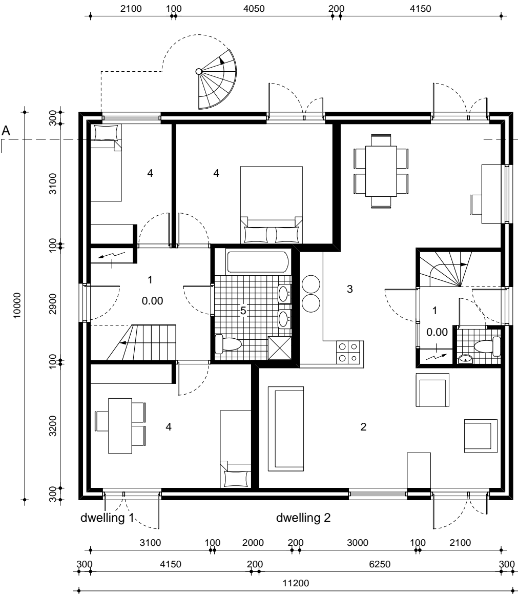
Ground floor 1:100
