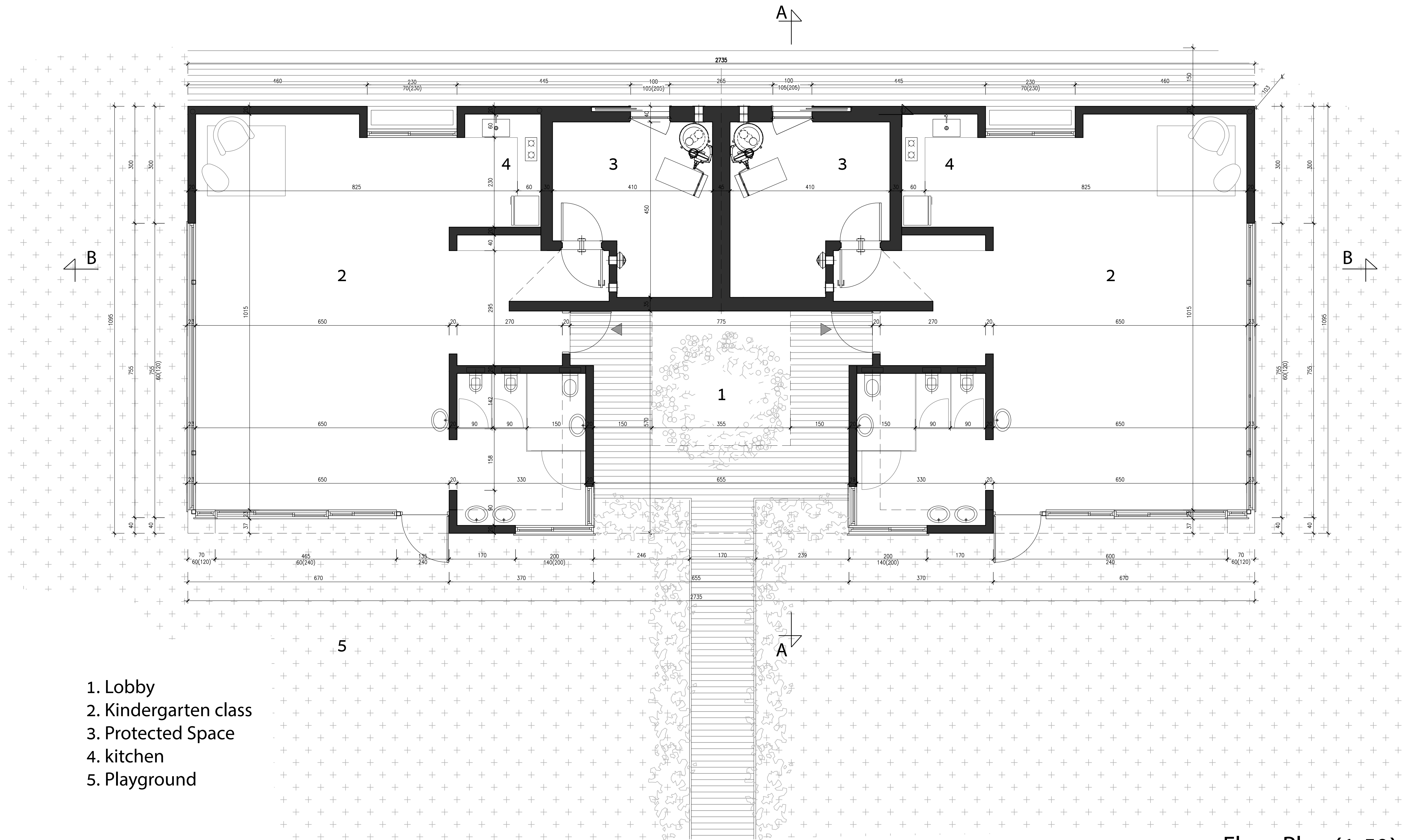
Floor Plan (1:50)
