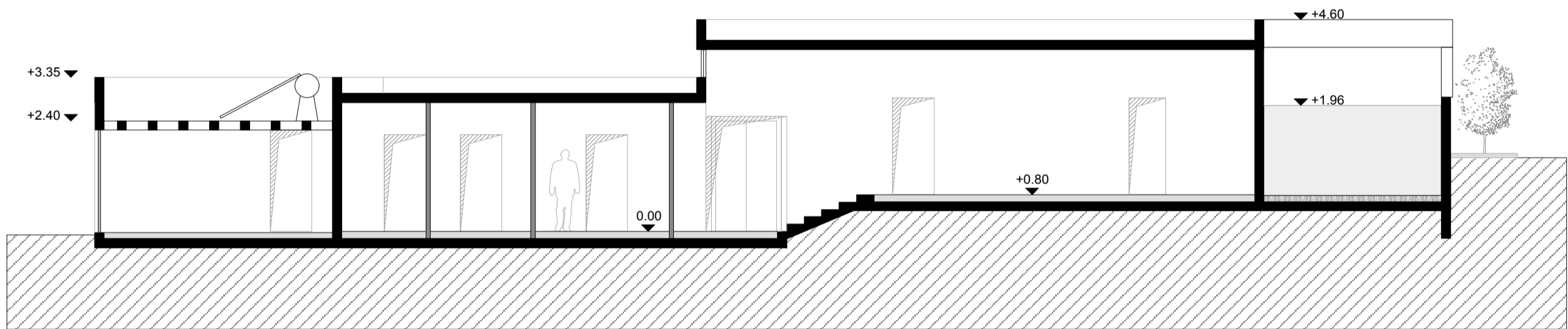
Section C-C
