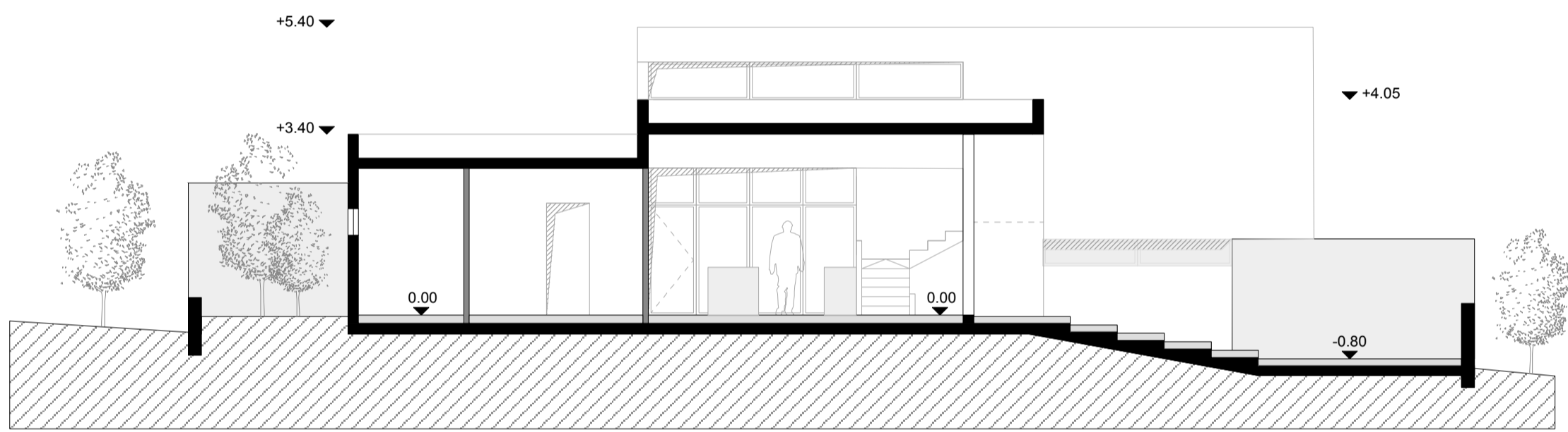
Section C-C
