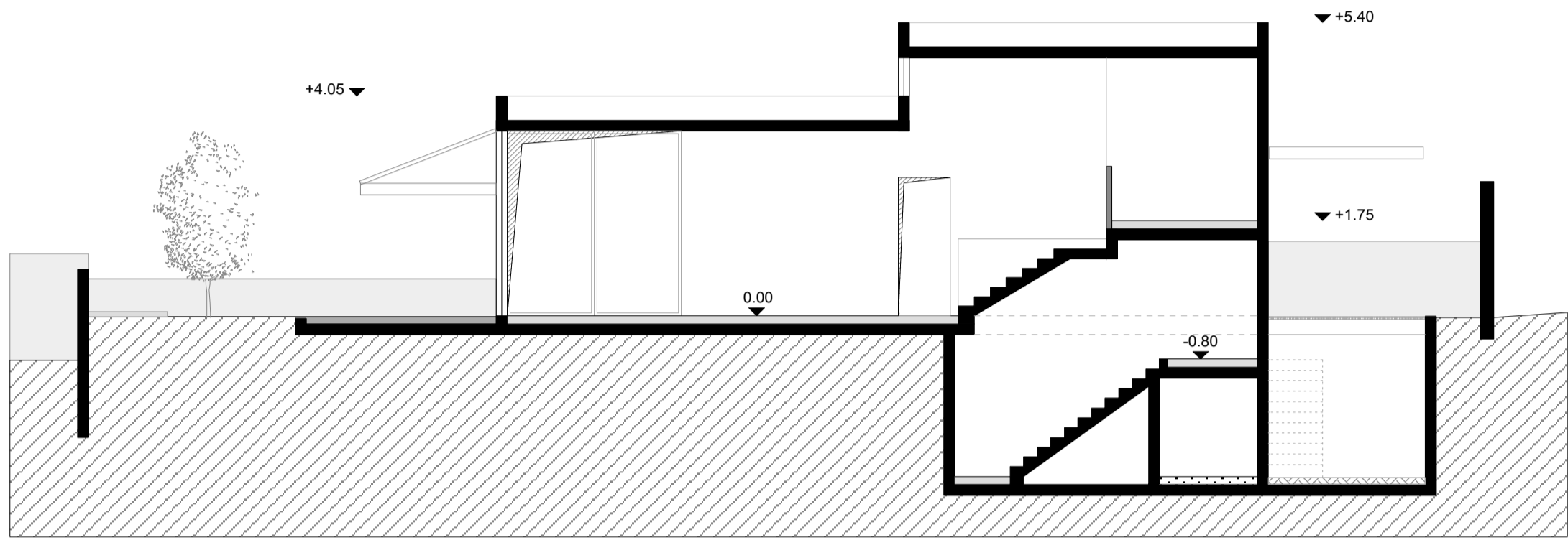
Section B-B
