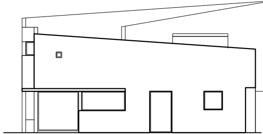
East elevation 1:200
