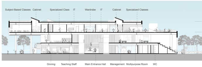
SECTION B-B SCALE 1-200
