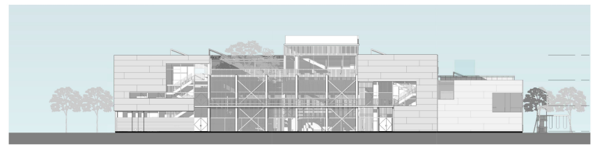
SOUTH EAST FAÇADE SCALE 1-200
