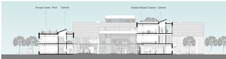
SECTION C-C SCALE 1-200
