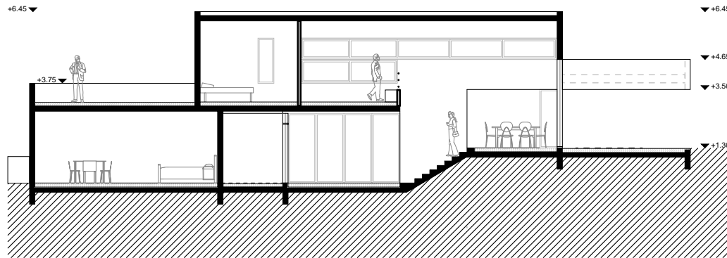
Section B-B
