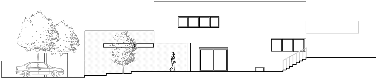
South facade
