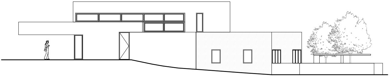
North facade
