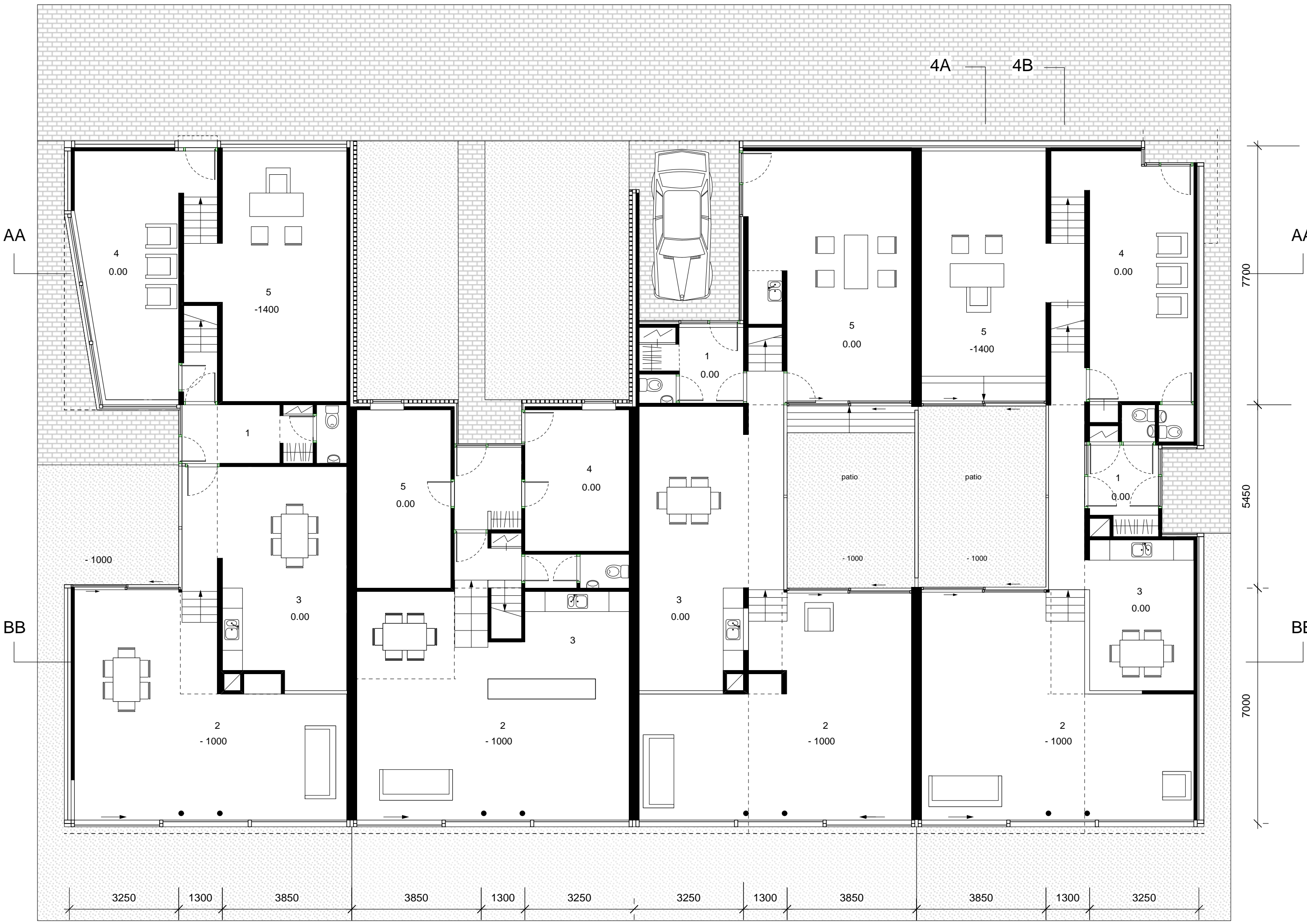
dwelling 1 dwelling 2 dwelling 3 dwelling 4 Ground floor 1:100
