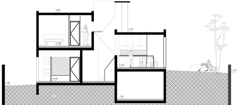
section 1:200
