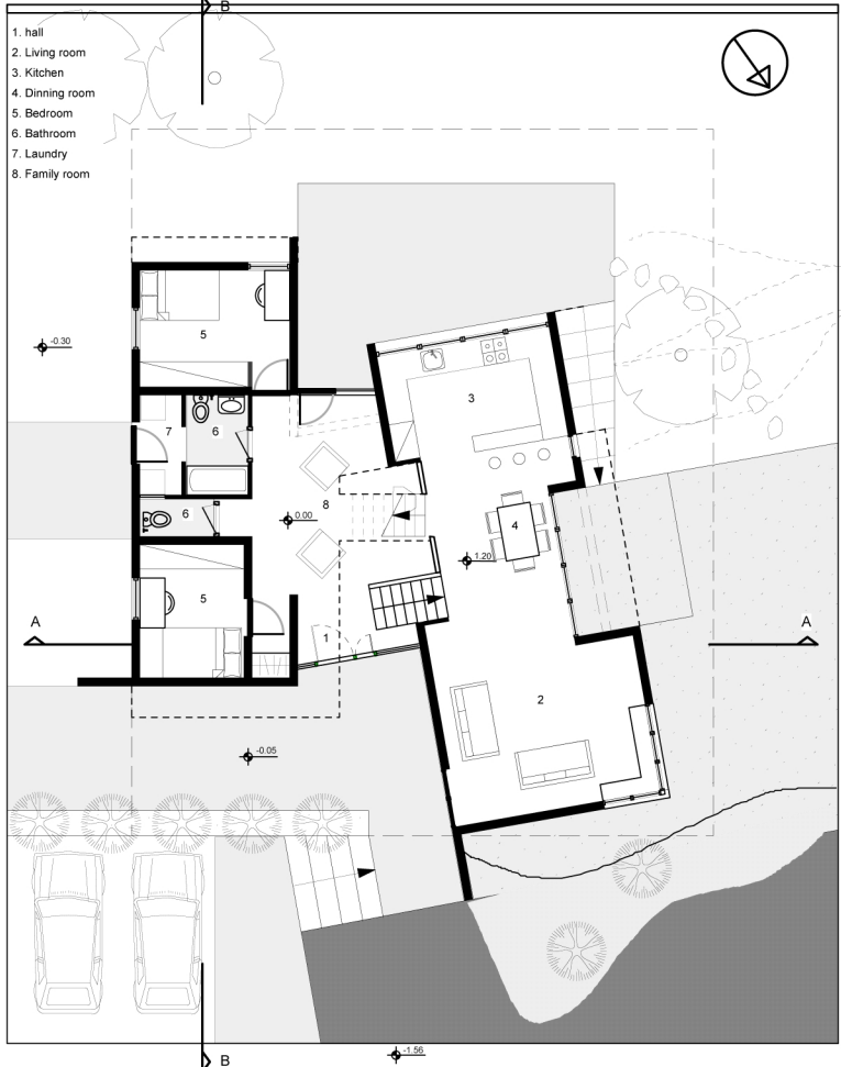
lower levels 1:200
